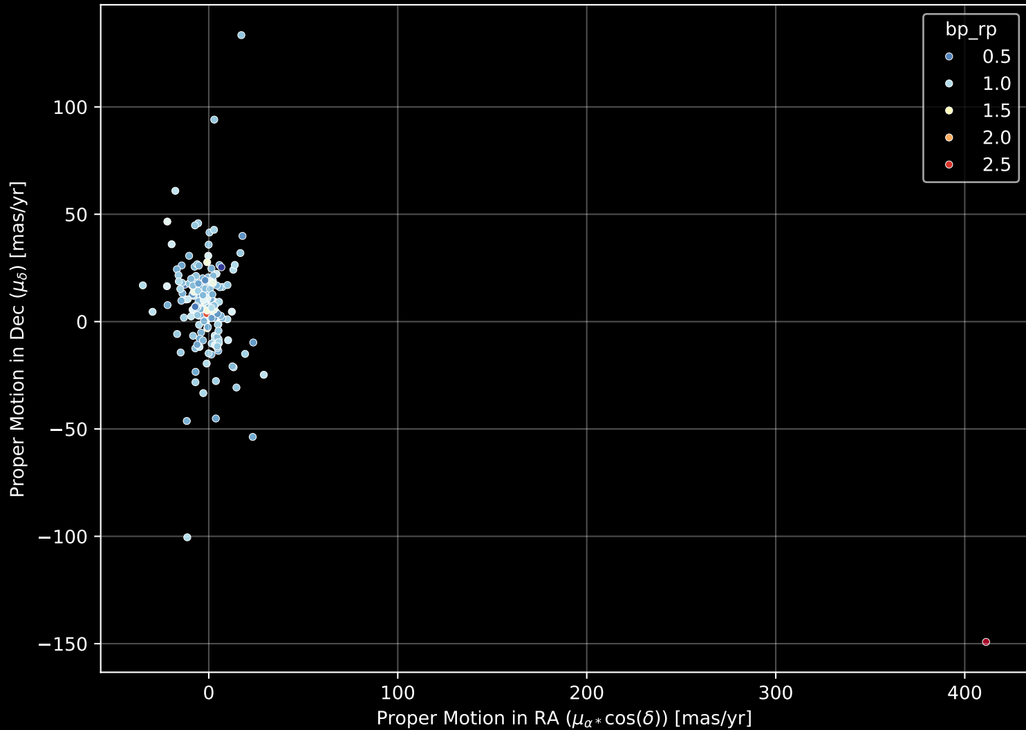
GALAH DR4 Field: [7189] Proper Motion Diagram (n= 202)
