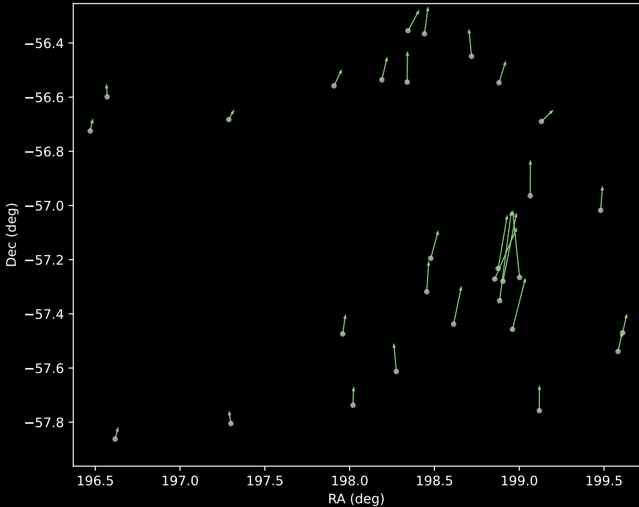
GALAH DR4 Cluster 5 Proper Motion Vectors (n=30)
