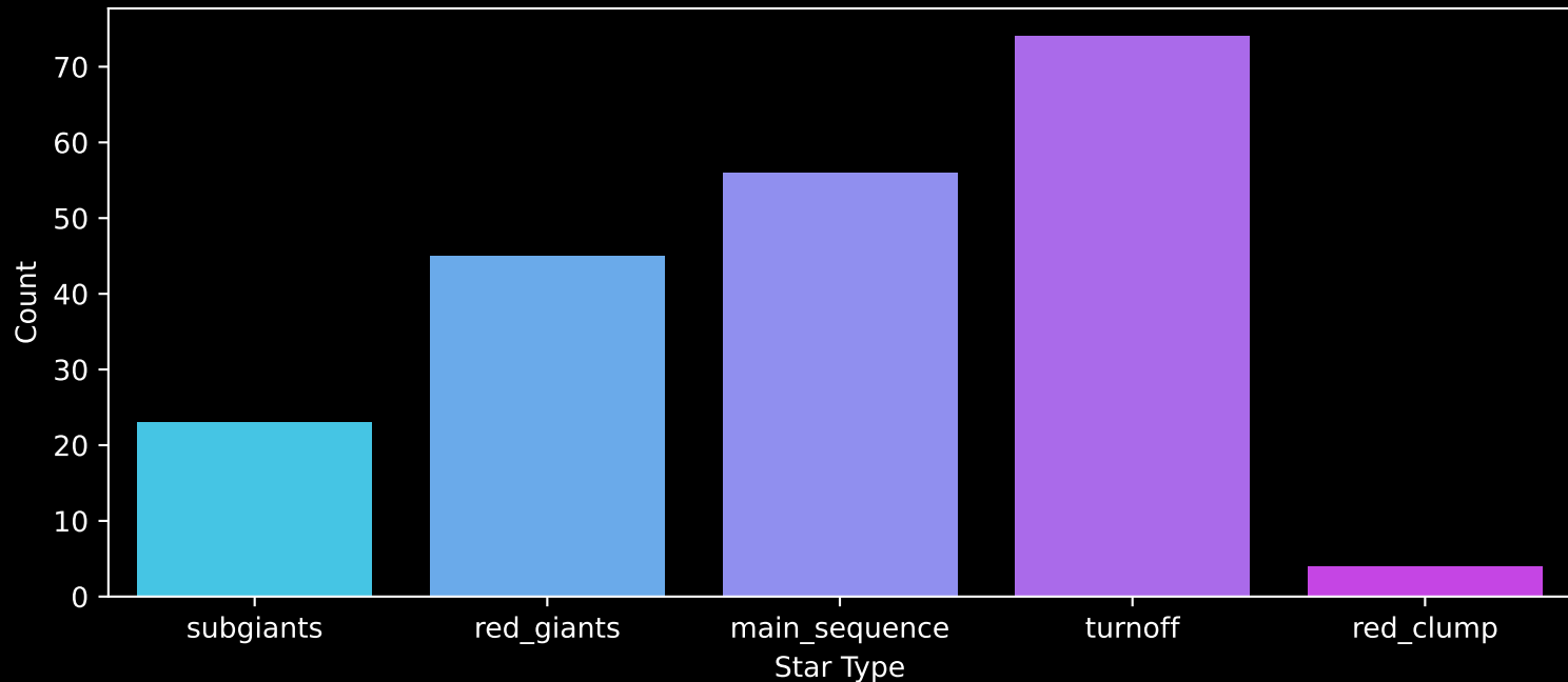
GALAH DR4 Field: [7189] Count plot of Star Type
