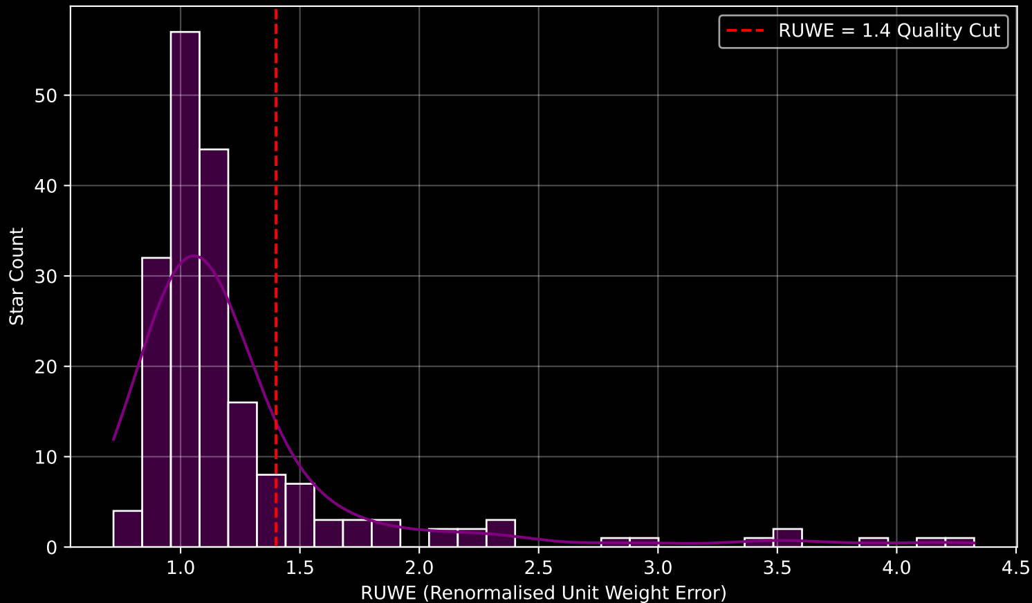
GALAH DR4 Field [7189] RUWE Distribution (n= 192)
