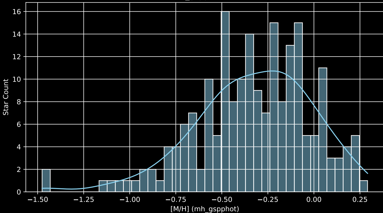
GALAH DR4 Field: [7189] [M/H] (mh_gspphot) (n= 202)
